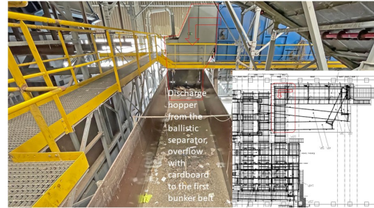
Overflow (cardboard) from the ballistic separator
